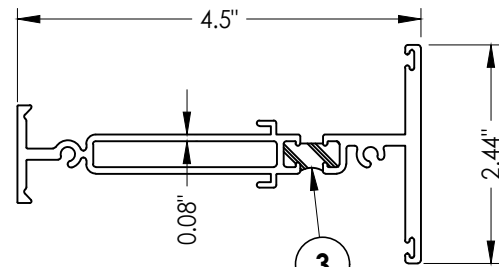
6 MULLION
