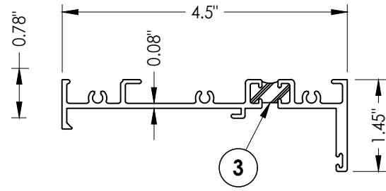
2 BLOCK FRAME
