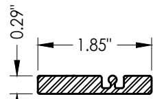
12 SHEAR BLOCK
