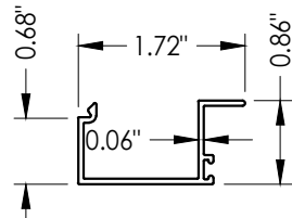
10 GLASS STOP 5/16", 7/16", 9/16" OPERABLE PANEL
