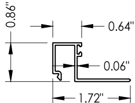
8 GLASS STOP 1-1/4" OPERABLE PANEL
